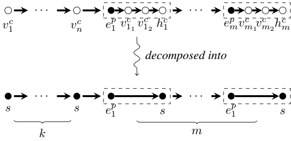
Figure 3: The construction for the proof of Prop. 1 in our earlier work (Lin and Bercher 2021). The constructed domain contains only one primitive task (action) s .
